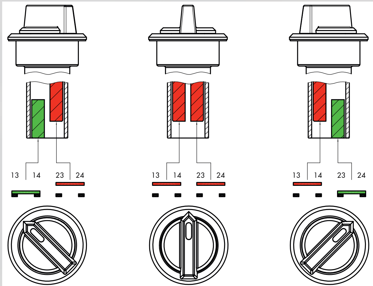
illustration of two-piece plunger
