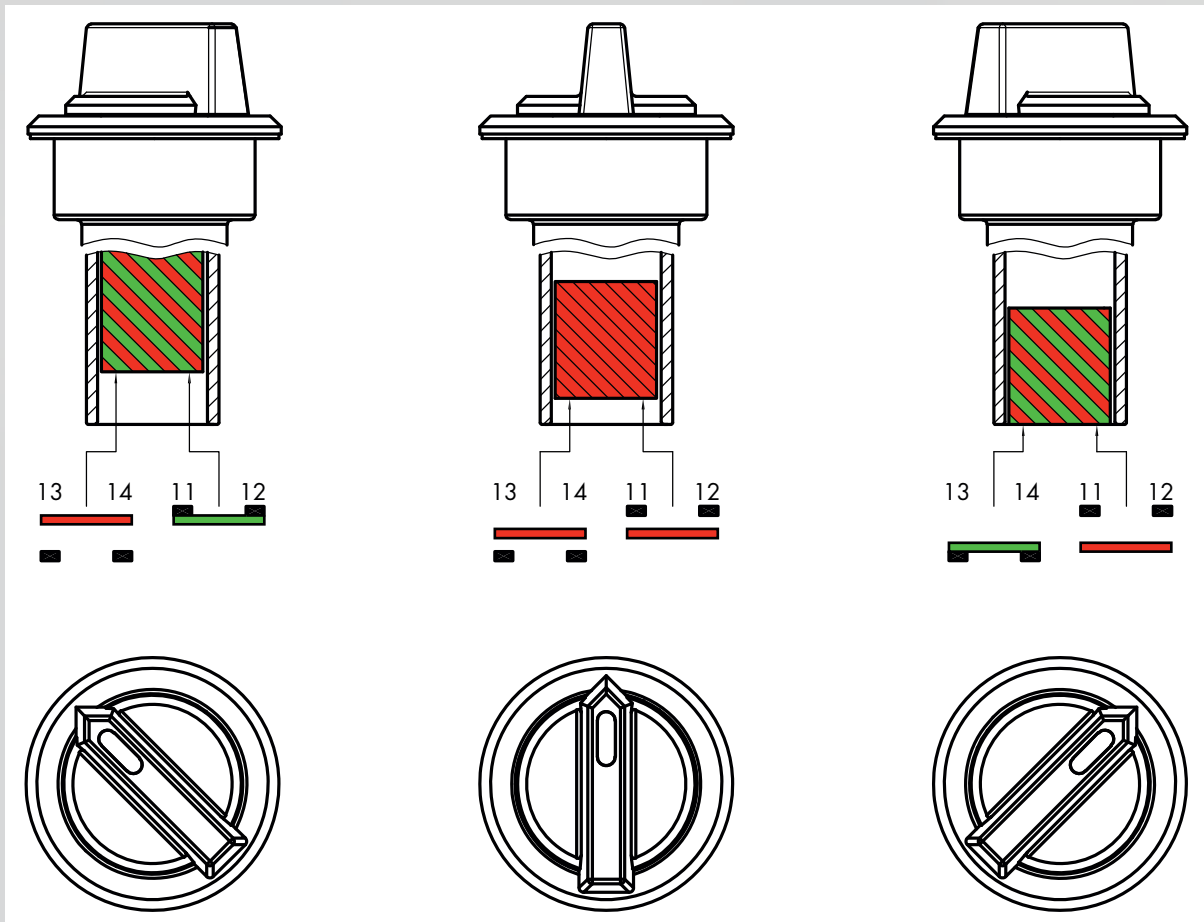
illustration of one-piece plunger
